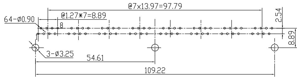
PC BOARD LAYOUT THICKNESS=1.6mm
